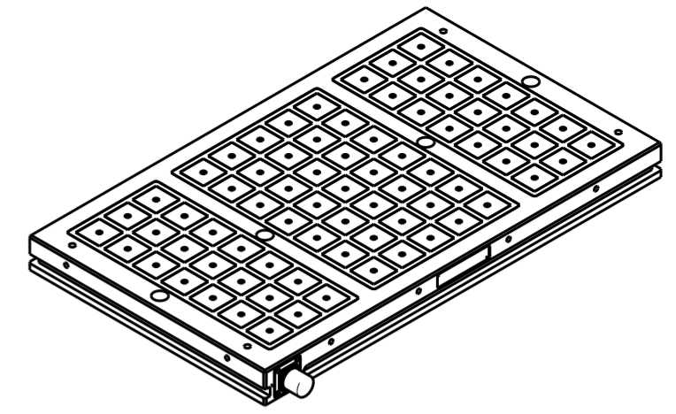
Isometric view (1:10)
